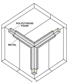
Interior Corner Batten
